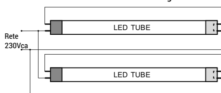
Double tube wiring
