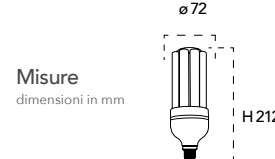
Lampada LED classe A+ E27 LOWBAY 27W 230V
